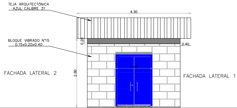
FACHADA PRINCIPAL CASETA
